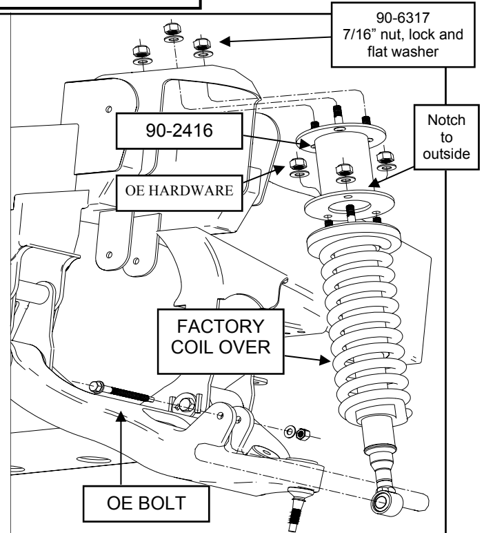
Illustration 1b With coil spacer
