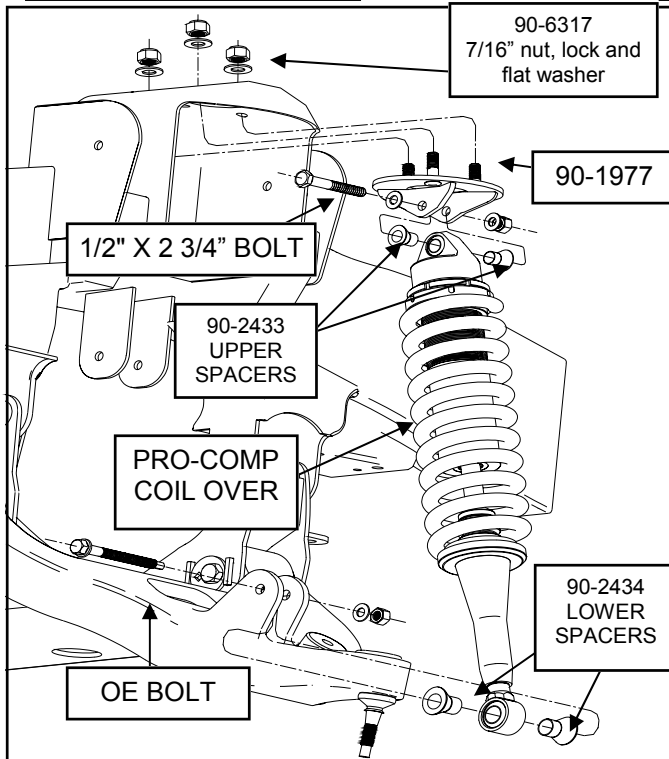
Illustration 1a With coil over
